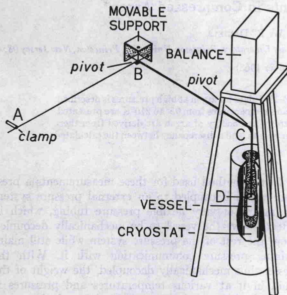
FIG. 1. Weighing apparatus.
